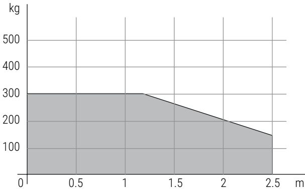
BE20/200/HS
